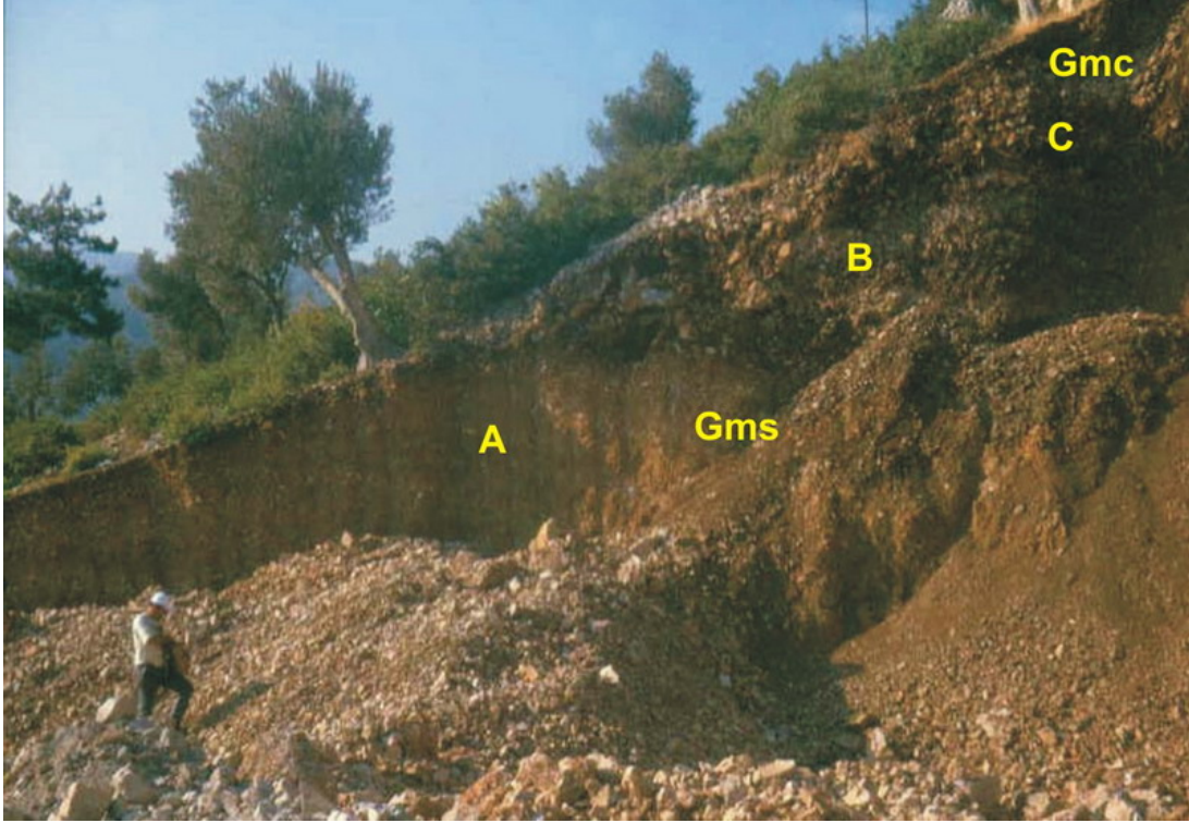
Figure 4. The facies characteristics of the Karaman colluvial deposits which are adjacent to the Karaman fault. A, B and C levels in the Karaman sequence were probably formed in the effect of three palaeoseismic activities, Gms (matrix supported conglomerate), Gmc (slip surfaces-bearing conglomerate).
